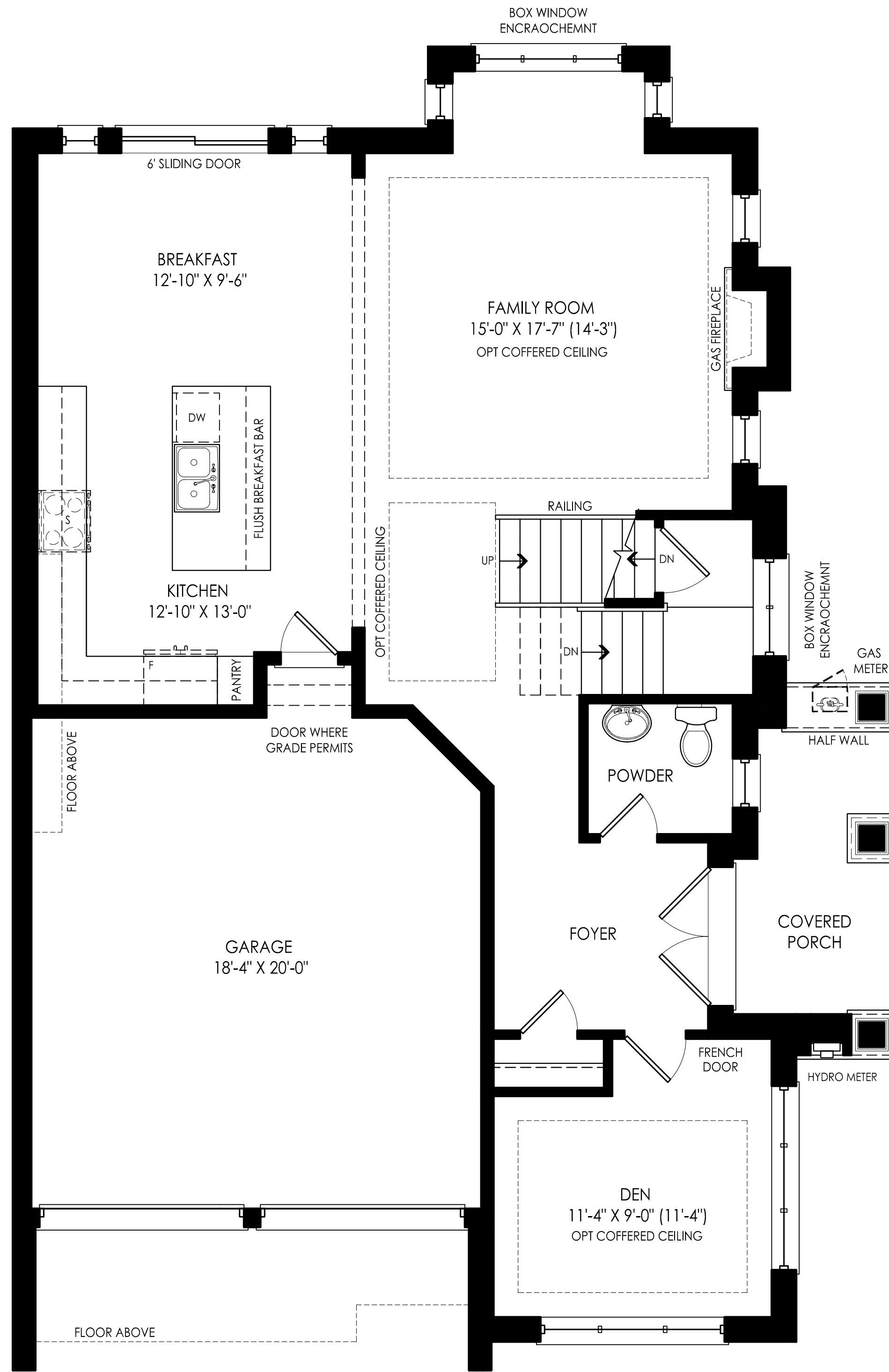
GROUND FLOOR ELEV. 'A'
