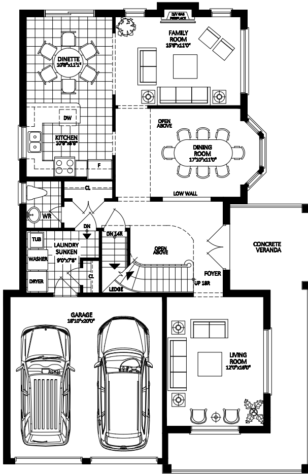
Main Floor
